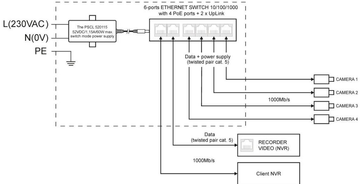
Fig. 1. Block diagram.
