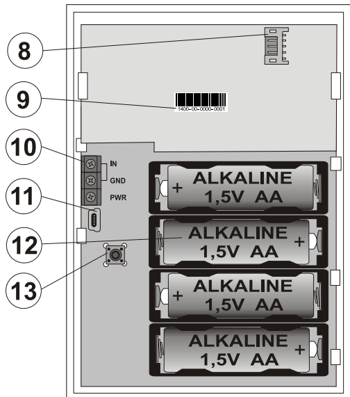
Figure: 8 – control segment connector; 9 – production code; 10 – terminals; 11 – mini USB connector; 12 – batteries; 13 – tamper contact
