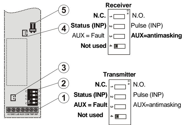
Fig. 3 Radio transmitter (matched transmitter and receiver):
