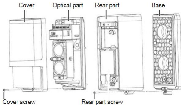
Fig. 1 Barrier parts (identical for transmitter and receiver)
