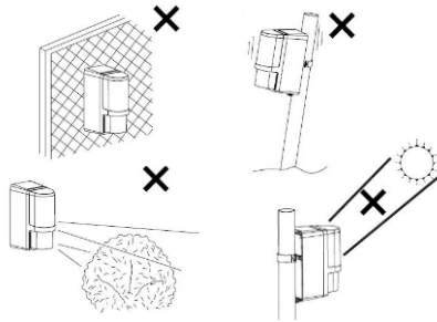
Fig. 1 Undesirable locations
